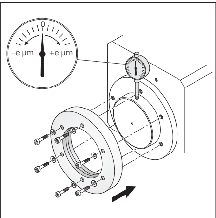
Centering via a centering collar
