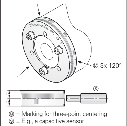
Three-point centering for the ERA
