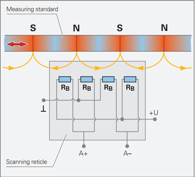
Magnetoresistive scanning principle
