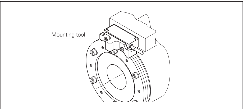
Mounting the scanning head for the ECA 4000/ERA 4000
