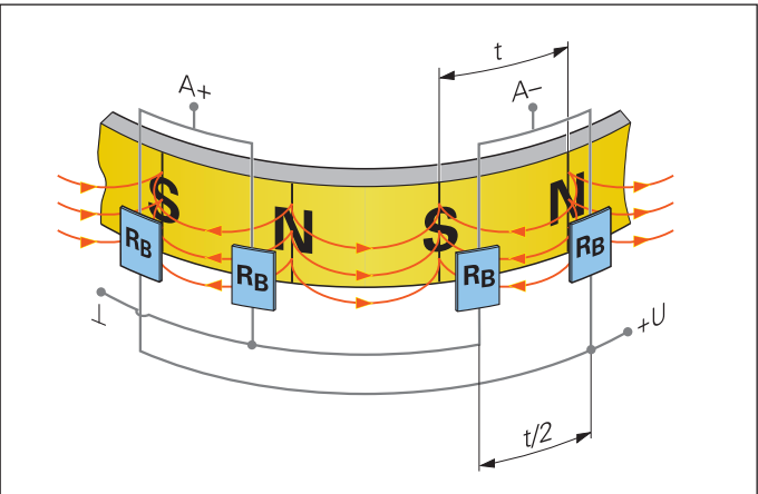
Magnetoresistive scanning principle
